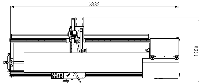
Standard size machine for a 2.5mtr roll
